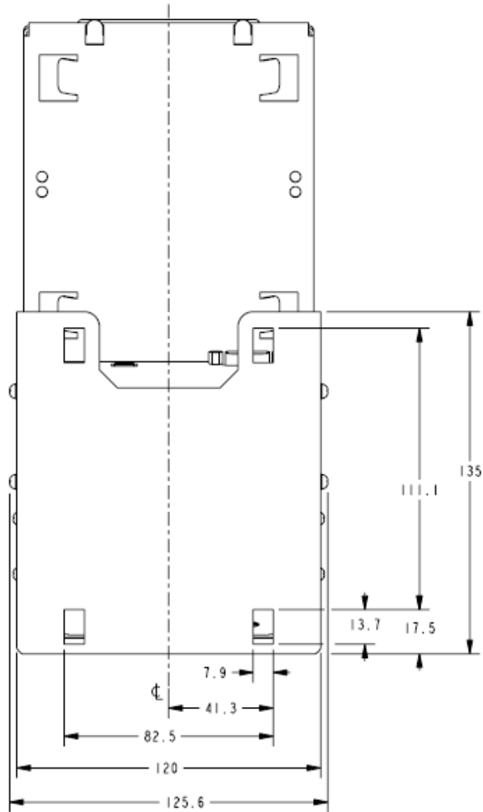
Figure 10: Back View
