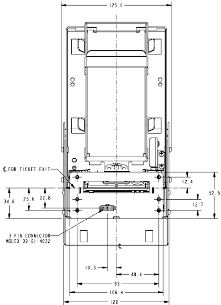
Figure 9: Front View
