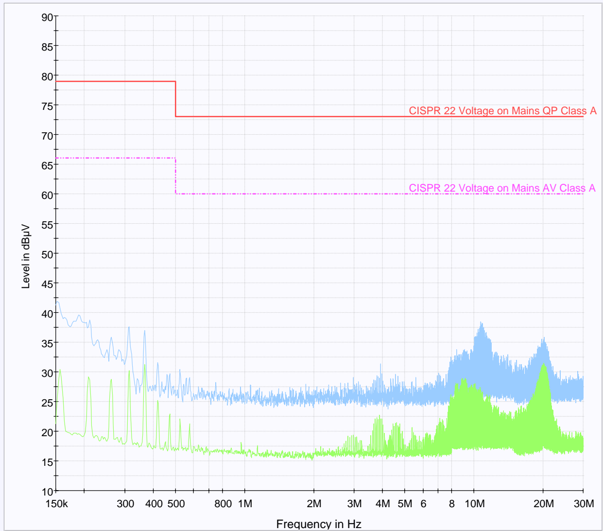
Neutral- 120V/60Hz
