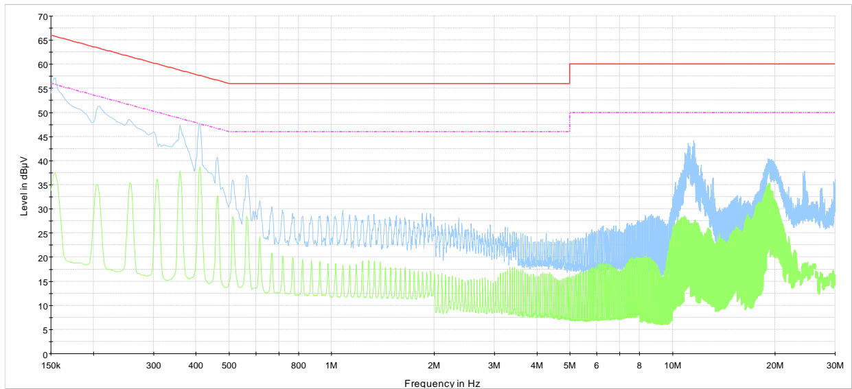
1R188613 - October 27, 2011 - 230 VAC, 50 Hz - Phase — CISPR 22 Mains QP Class B LimitLine - - - CISPR 22 Mains AV Class B LimitLine — Preview Result 1-PK+ — Preview Result 2-AVG
