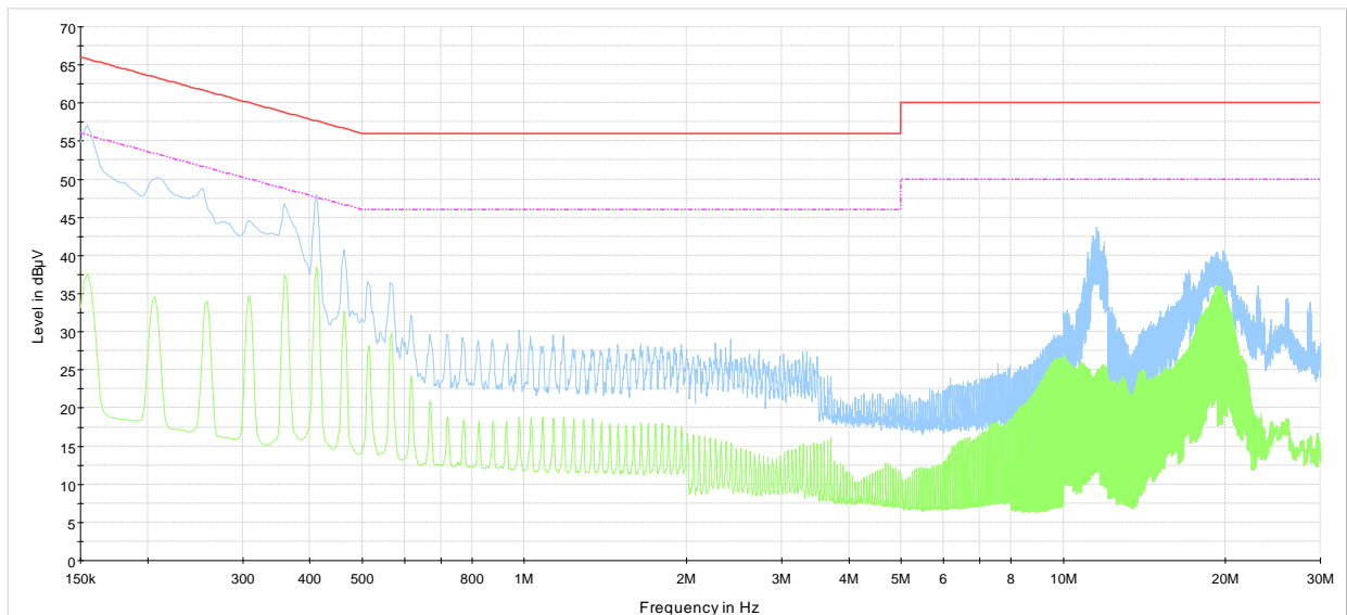
1R188613 - October 27, 2011 - 230 VAC, 50 Hz - Neutral — CISPR 22 Mains OP Class B LimitLine - - - CISPR 22 Mains AV Class B LimitLine — Preview Result 1-PK+ — Preview Result 2-AVG
