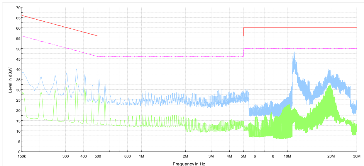
1R188613 - October 27, 2011 - 120 VAC, 60 Hz - Neutral — CISPR 22 Mains OP Class B LimitLine - - - CISPR 22 Mains AV Class B LimitLine — Preview Result 1-PK+ — Preview Result 2-AVG
